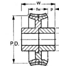
Two piece gear Type G4
