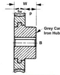
Gear with cast iron hub Type G2
