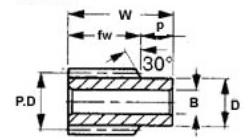
Worm with hub - no set screw Type W2
