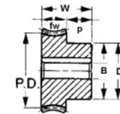
Gear with hub - No setscrew Type G3
