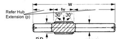
Worm with integral shaft Type W5
