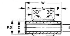
Worm with double hub Type W3 (no set screw)
