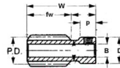
Worm with hub and set screw Type W1
