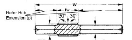
Worm with integral shaft Type W5
