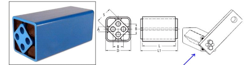
MOUNTING Bolted Lever Arm on Inner Square: Connection with 2 or 4 shaft screws across the inner square profile, or by means of set screws directly on the square (the customer-side thread tapping is required).
